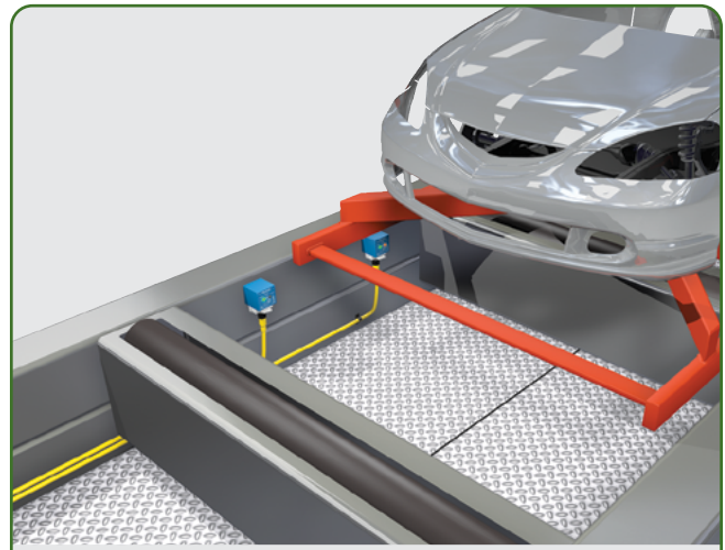
Automotive application - Two general purpose VersaCubes detecting skid position in a body shop.
