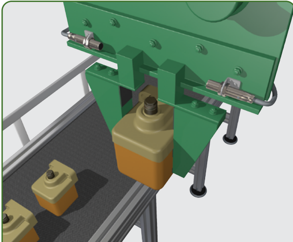
Gripper application - Two 871C inductive sensors detecting open position of gripper jaws
