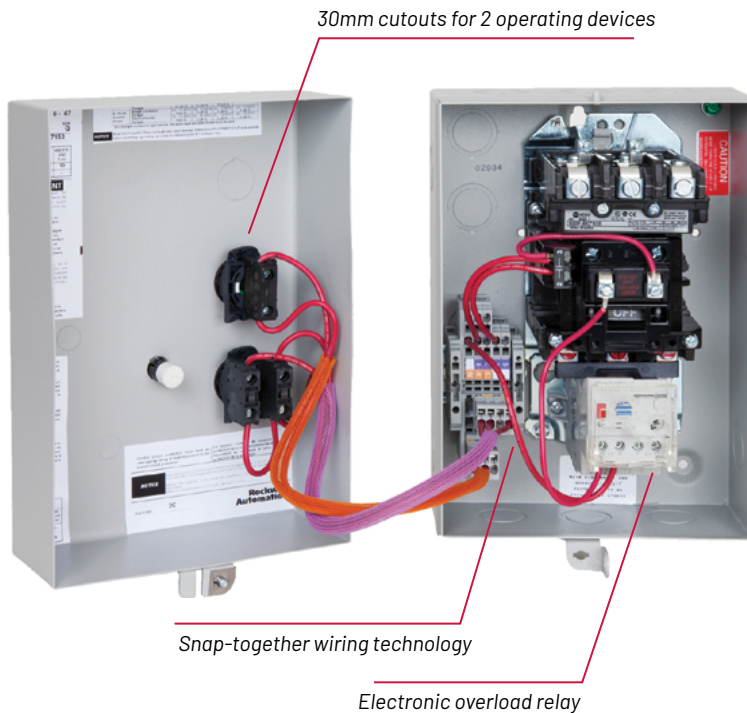
509 Enclosed Starter
