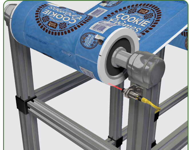
Roll detection - A 42CM LaserSight monitors a roll of film to indicate low film level.
