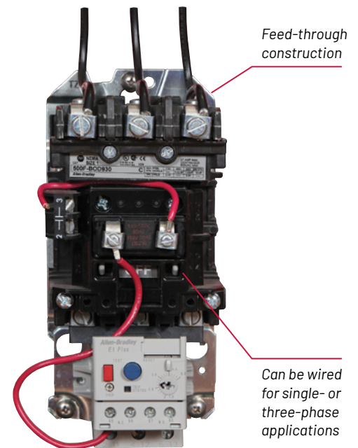
509 Open Starter
