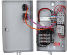
IEC STARTERS
