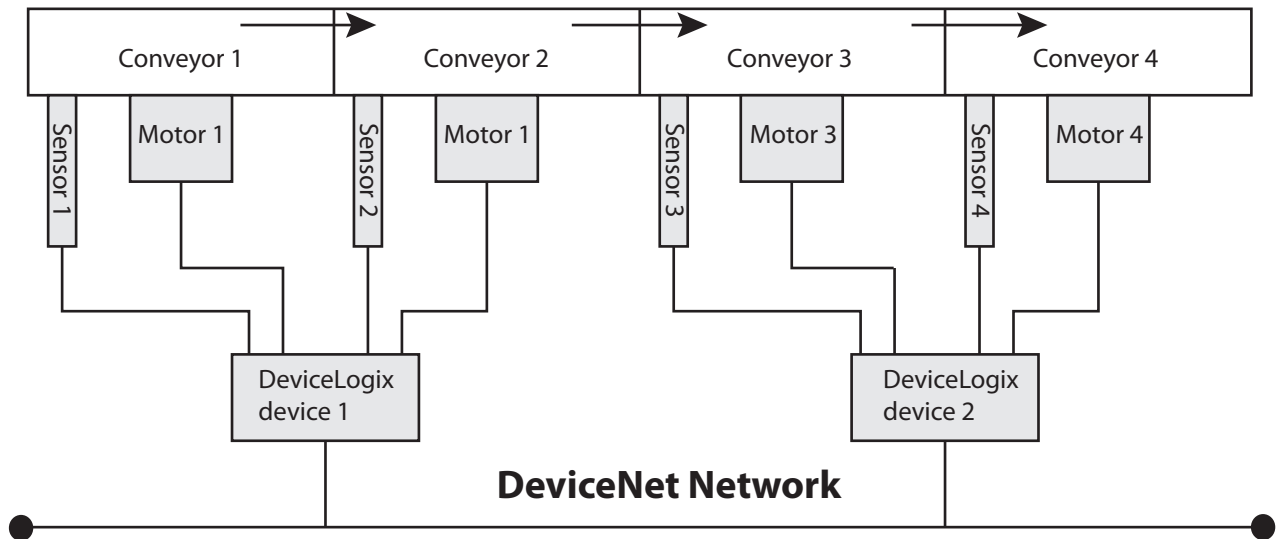
Figure 4 - Typical Material Handling Application
