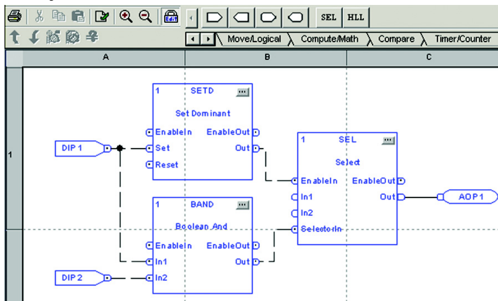
Figure 1 - Function Block Diagram
