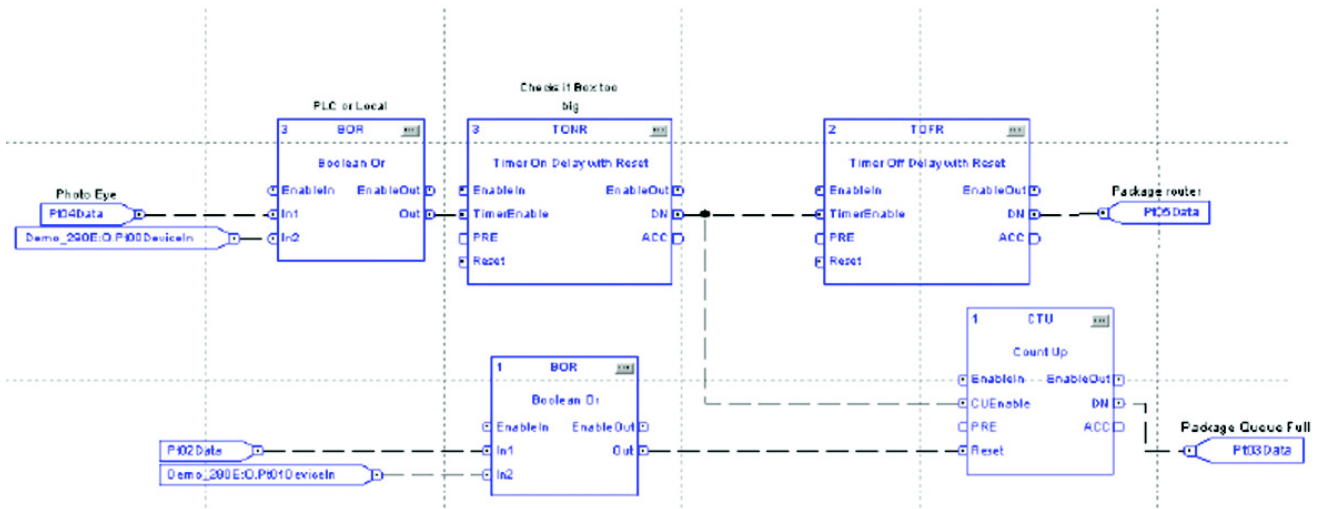
Figure 6 - Completed DeviceLogix Functionality for Material Handling Application
