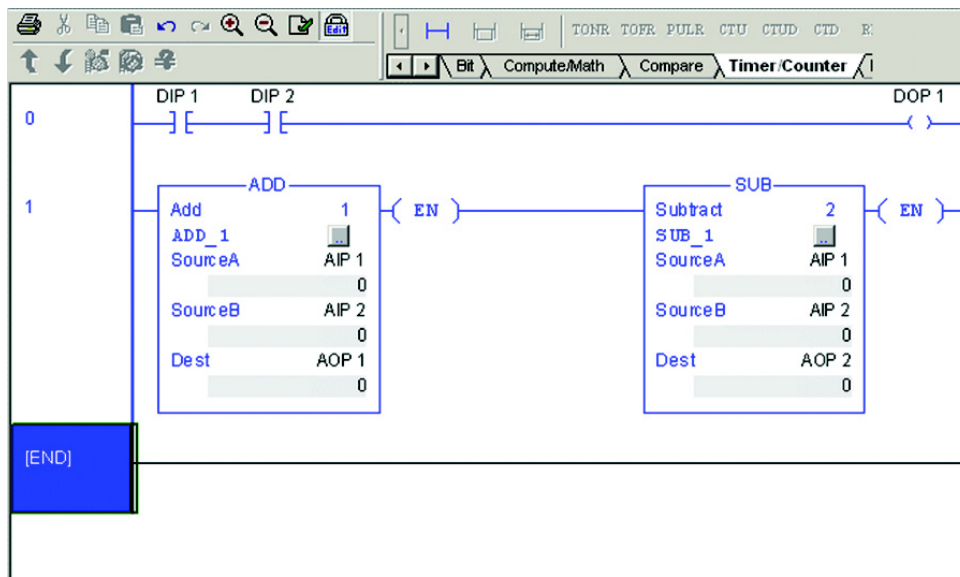
Figure 2 - Ladder Logic Diagram
