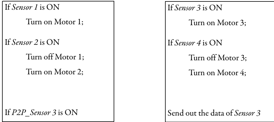
Figure 6 - Completed DeviceLogix Functionality for Material Handling Application
