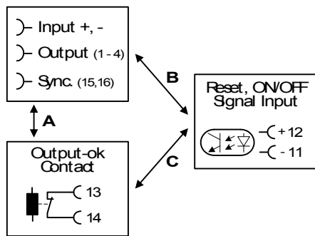
Figure 12: Dielectric strength
