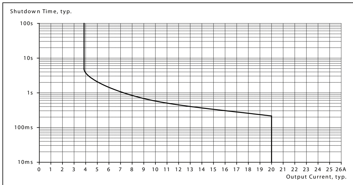
Figure 5: Shutdown characteristics
