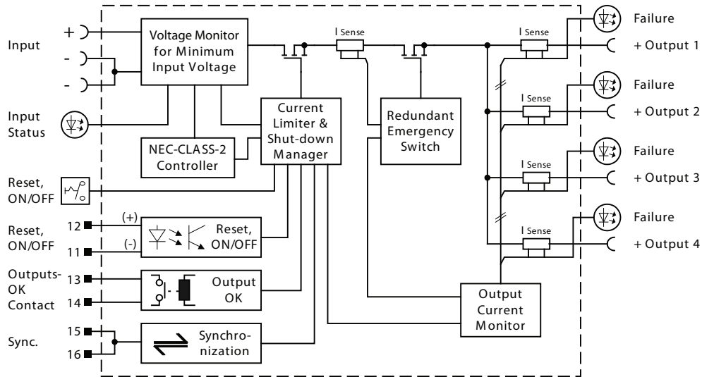
Figure 9: Functional Diagram
