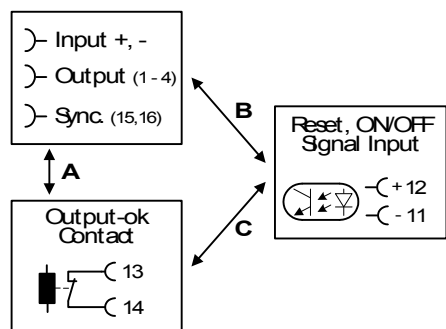
Figure 12: Dielectric strength
