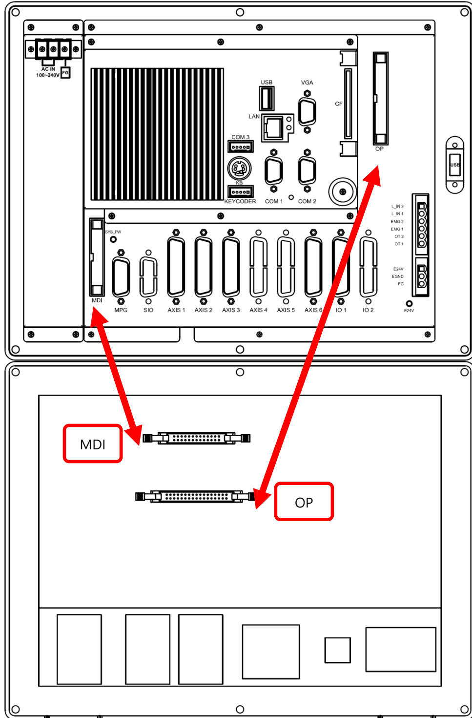
T/M 6□8A Wiring on controller
