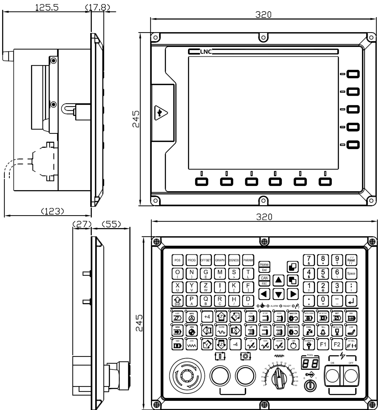
M 6□8A Dimension
