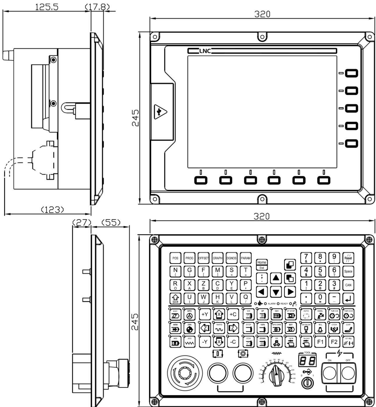
T 6□8A Dimension
