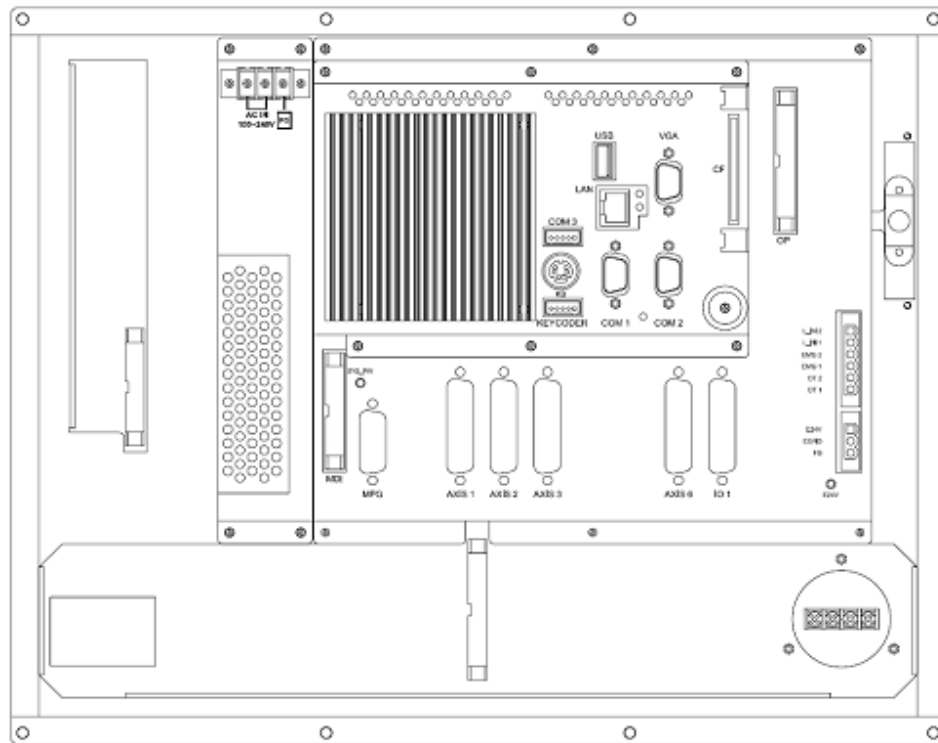
T 518A Controller Back View
