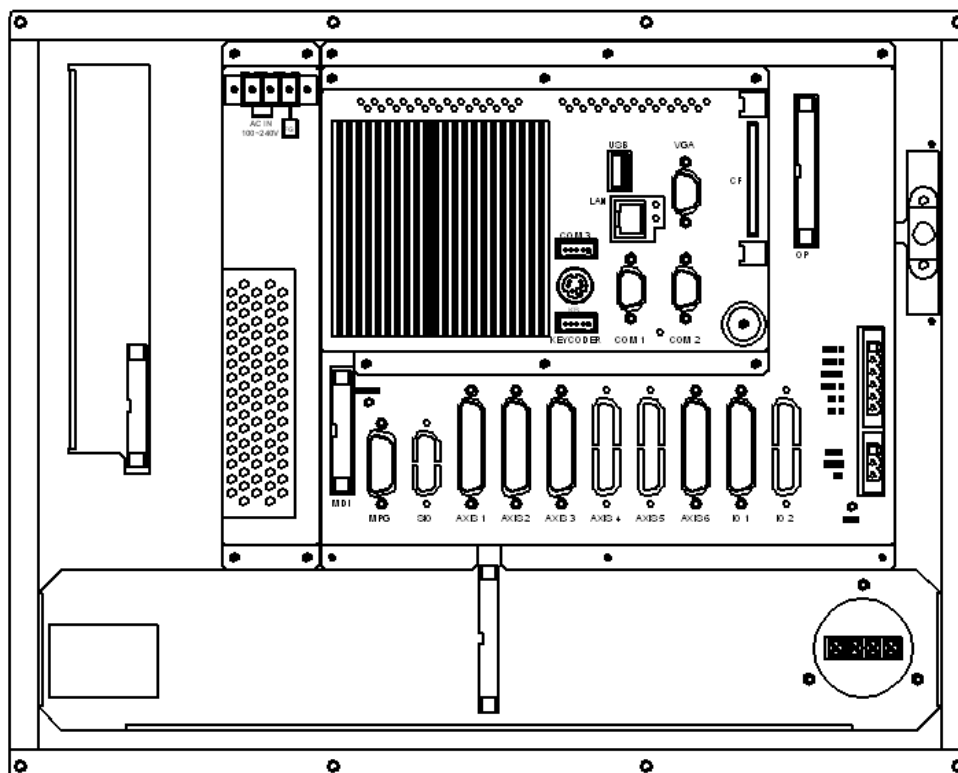
T 568A Controller Back View
