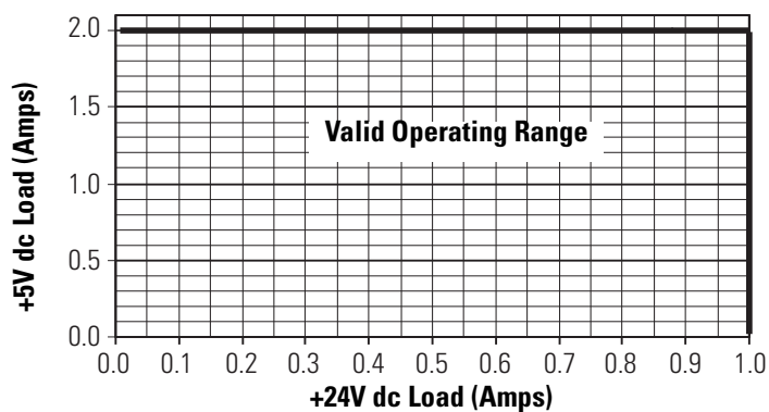
Figure F.1 1769-PA2 Current with +24V dc User Load = 0A
