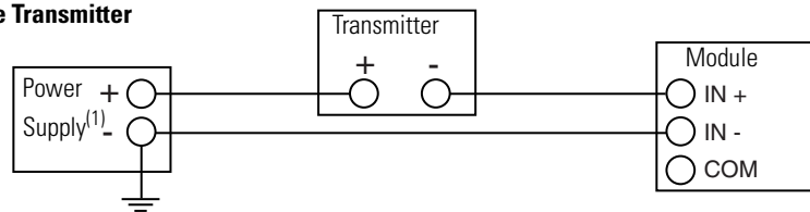
Figure 3.36 Single-ended Sensor/Transmitter Types
