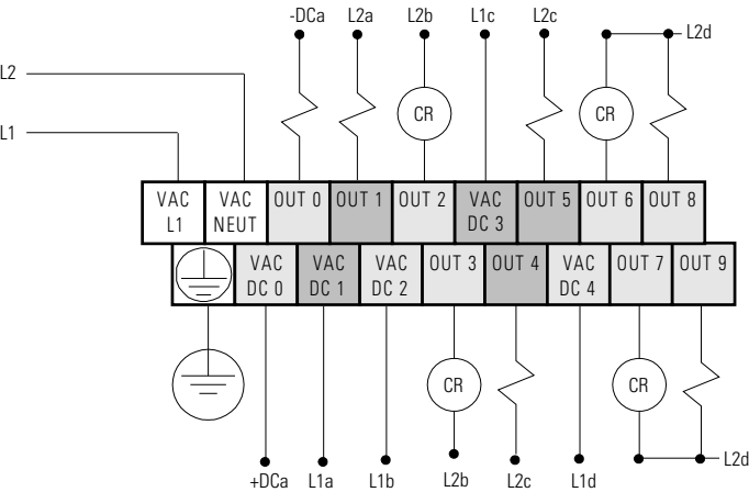
Figure 3.12 1762-L24AWA, 1762-L24BWA, 1762-L24AWAR, and 1762-L24BWAR Output Wiring Diagram
