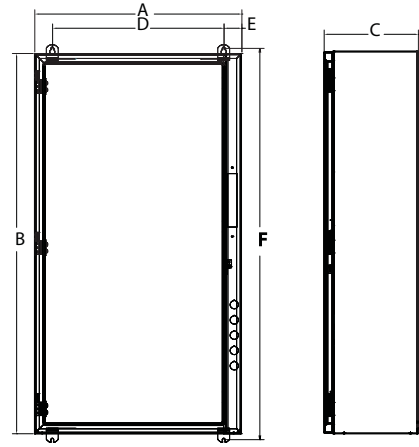
Figure 2 — Wall-Mount
